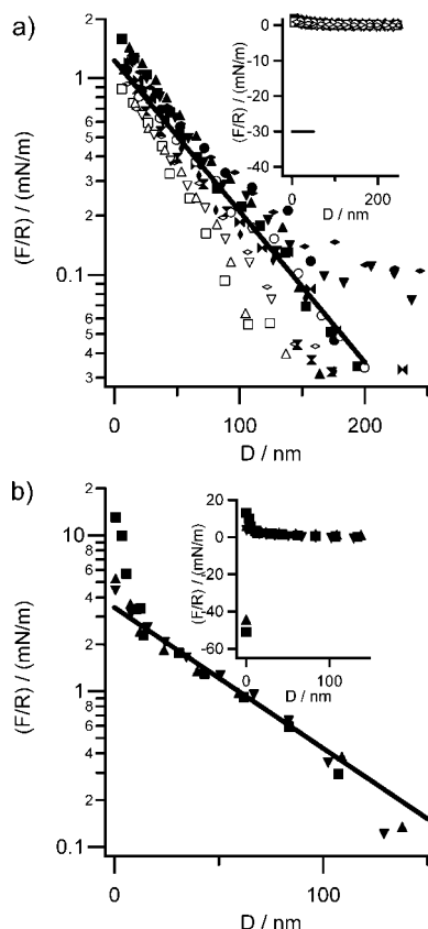
Figure 3. SFB control experiments. (a) Normal forces in water between mica surfaces that have been treated with an Ar/H 2 O plasma. Filled and open symbols respectively indicate force profiles measured at two different contact positions. The solid line shows a fit to eq 2, with \psi_0 = 130 mV and \kappa given by eq 3 with \rho_0 = 3 \times 10^{-5} M. (b) Normal forces in water between mica surfaces bearing a silane initiator layer. Symbols show measured force profiles. The solid line shows an exponential fit with the slope \kappa given by eq 3 with \rho_0 = 4 \times 10^{-5} M. The insets show the same force profiles as the main graphs, on linear scales, so that the jump into adhesive contact can be seen. Inset to part a: the measured lower limit on the magnitude of the pull-off force was 30 mN/m, marked by the solid line.
